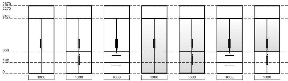
RH/LH STORAGE WALL ELEMENTS MODULI PARETE ATTREZZATA DX/SX
