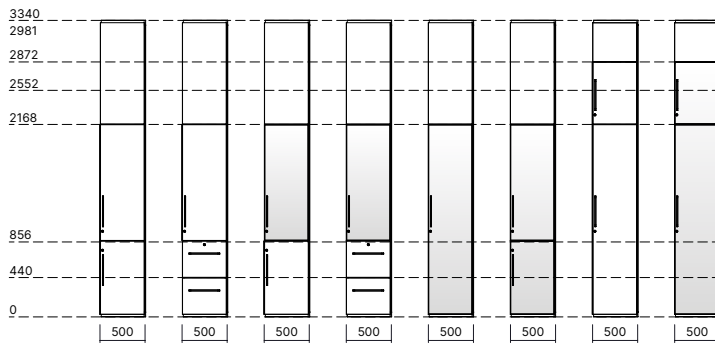
RH/LH STORAGE WALL ELEMENTS MODULI PARETE ATTREZZATA DX/SX
