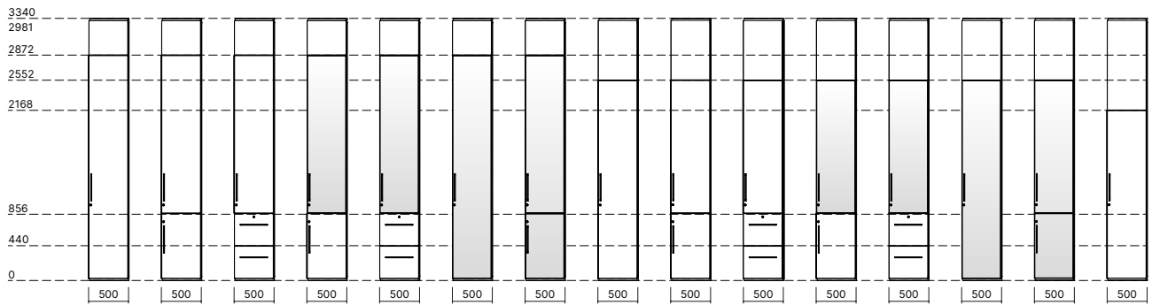
RH/LH STORAGE WALL ELEMENTS MODULI PARETE ATTREZZATA DX/SX
